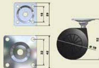
Rotary wheel Ø38 with square metal plate
