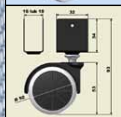
Rotary rubber wheel Ø50 with metal plate U16mm, U18mm
