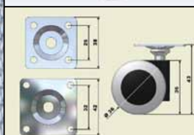
Rotary rubber wheel Ø35 with square metal plate
