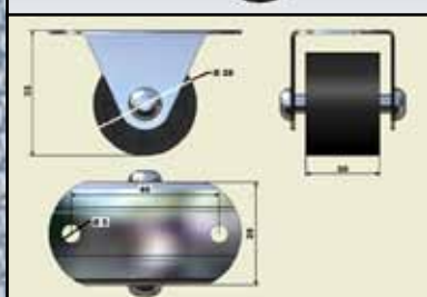
Straight rotary roll medium (plastic and rubber)
