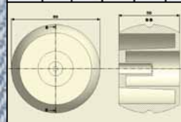
Foot fixed Ø80
