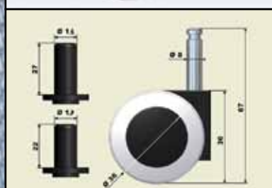
Rotary rubber wheel Ø35 with axle 8mm and sleeves H27
